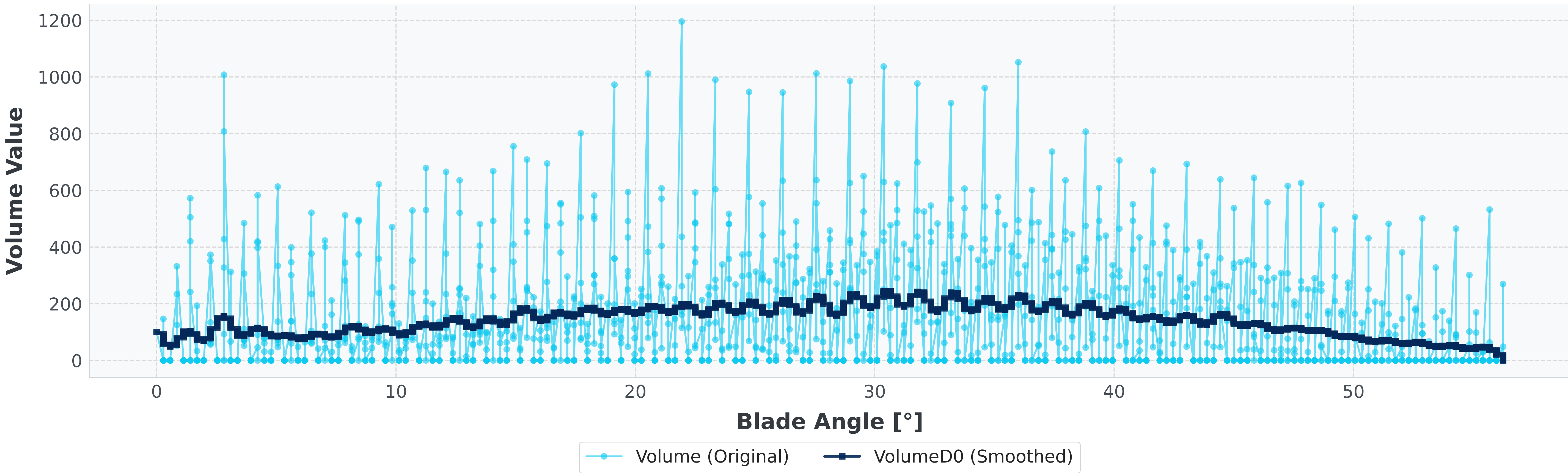
Cavity - Volume (BLD Phase Averaged)
